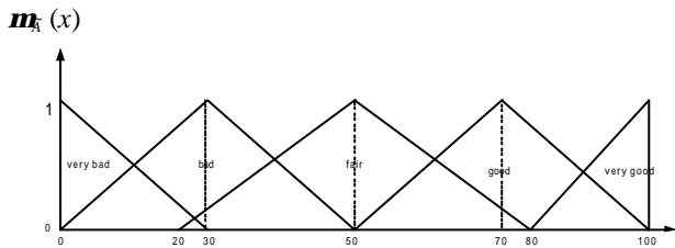
Fig. 2 Membership Function of the Five Levels of Linguistic Variables
