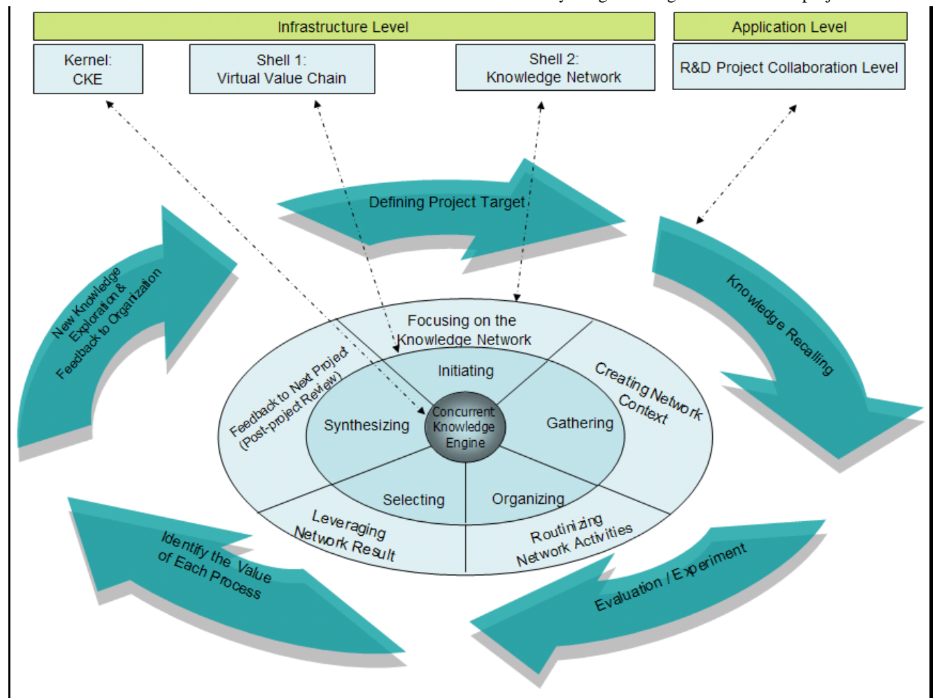
Figure 2: CKL model
