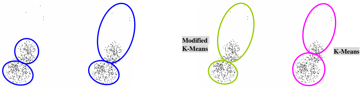
Figure 1 The comparison of dealing extreme value points by K-Means and modified K-Means
