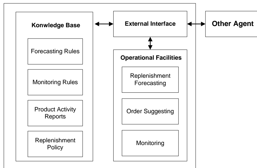
Figure 4. Architecture of a Forecasting Agent
