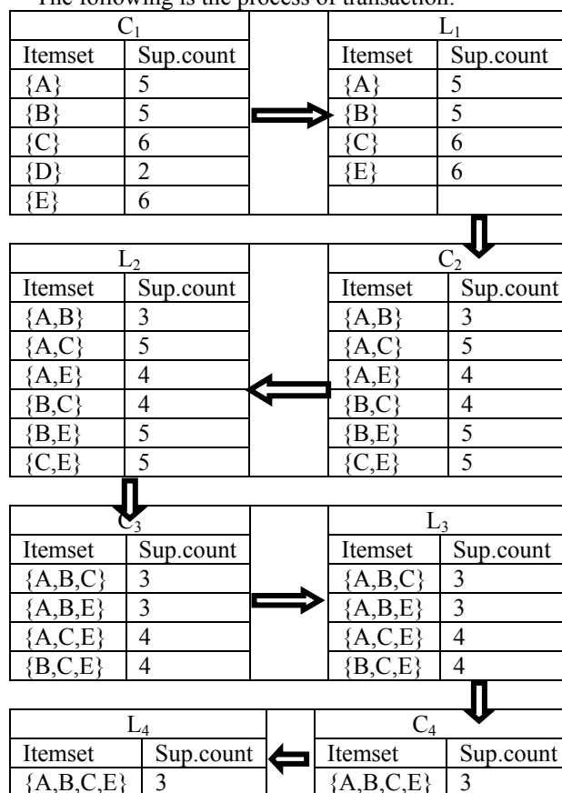
Fig.5: Generate of candidate and frequent itemsets
