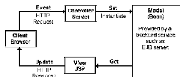
Figure1. M-V-C design pattern of eFramework
