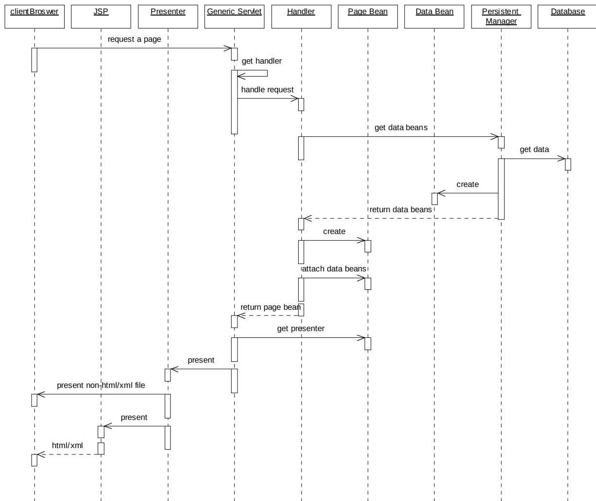
Figure2. M-V-C design pattern of eFramework
