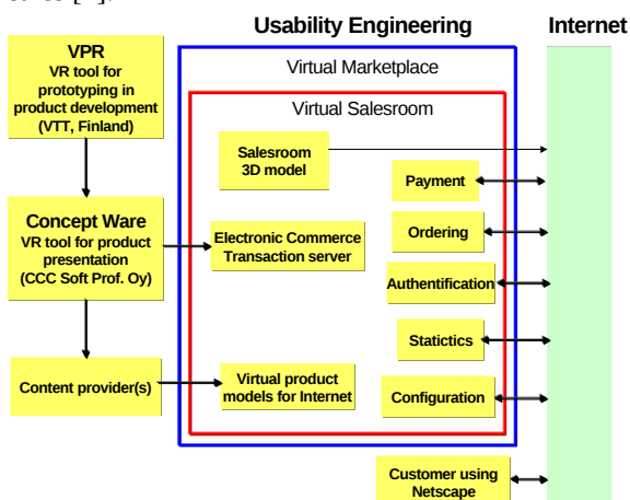
Fig.4. the proposed concept for Internet electronic commerce utilizing digital virtual product models in marketing and sales
