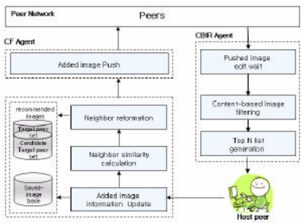
Figure 1. Personal Recommender Agent
