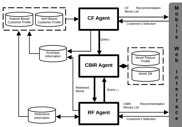
Figure 2. The architecture of MOBICORS-Movie
