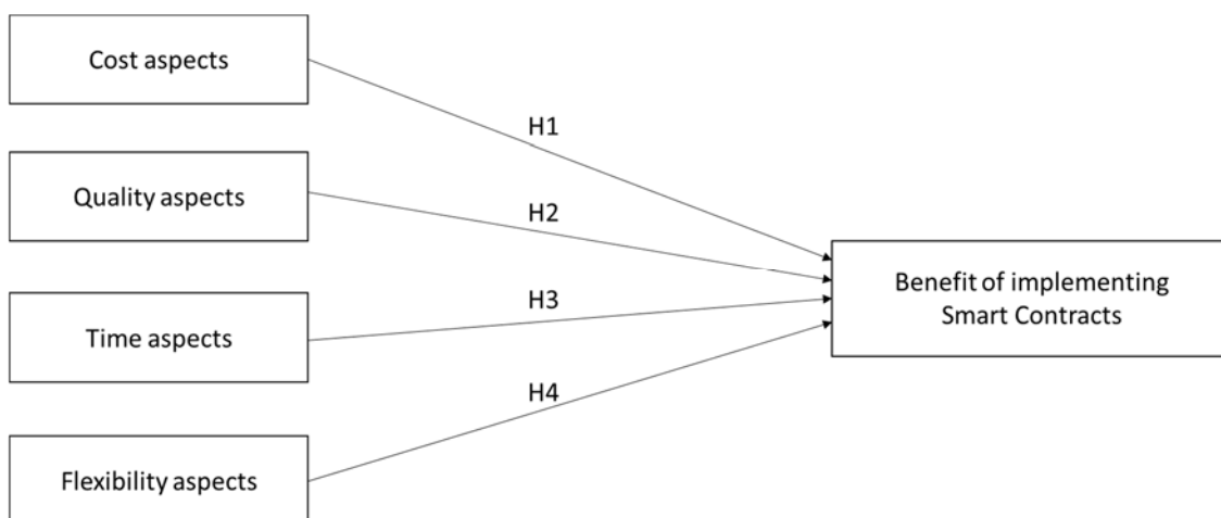
Figure 2: Research Model
